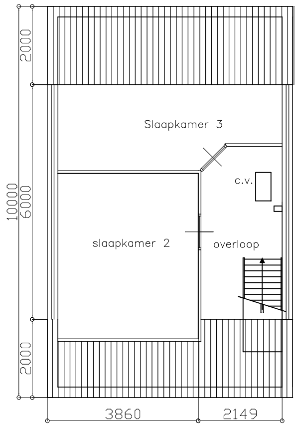
VERDIEPING.
